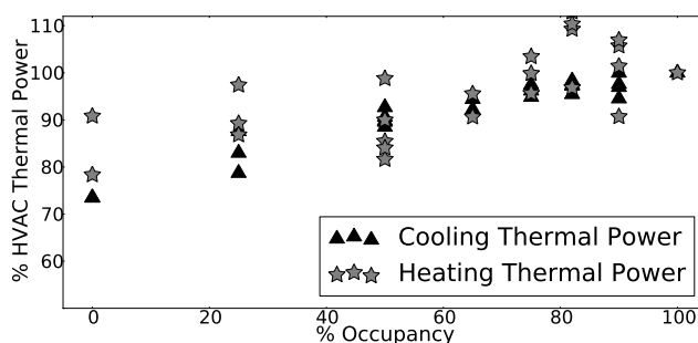
Figure 13: HVAC thermal power consumption with change in occupancy levels in the building
